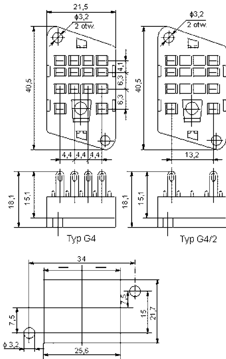
Socket G4/2 for panel mounting (R2 or R4 2C/O)
